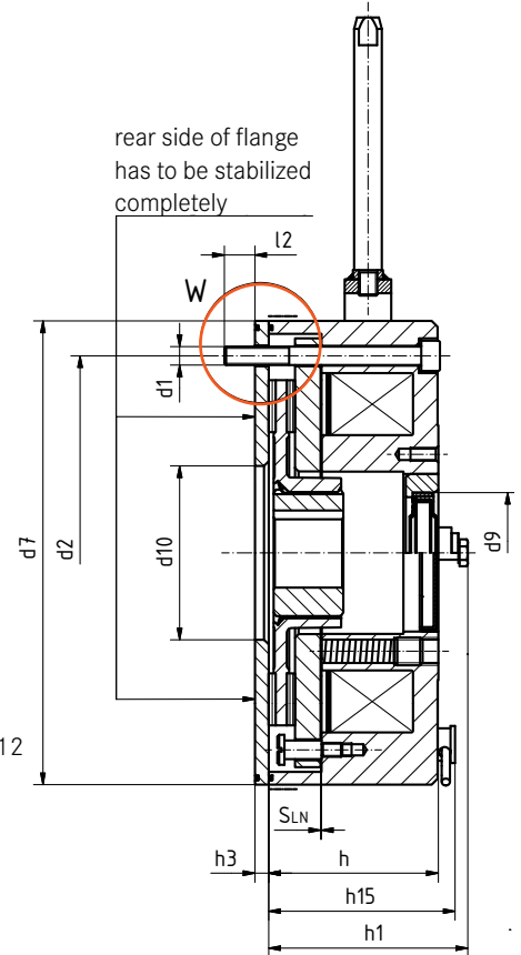
View W with centering
