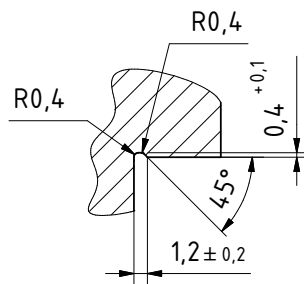
View Z Bearing shield
